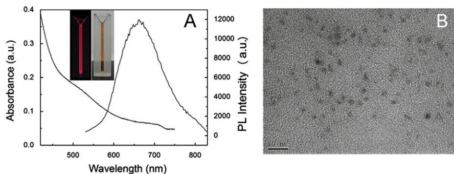
Fig. 1. (A) Fluorescence emission and UV-Visible absorption spectra of the BSA-AuNCs solution. Inset: photographs under ultraviolet light (left) and visible light (right) of the BSA-AuNCs solution. (B) HRTEM images of BSA-AuNCs.
