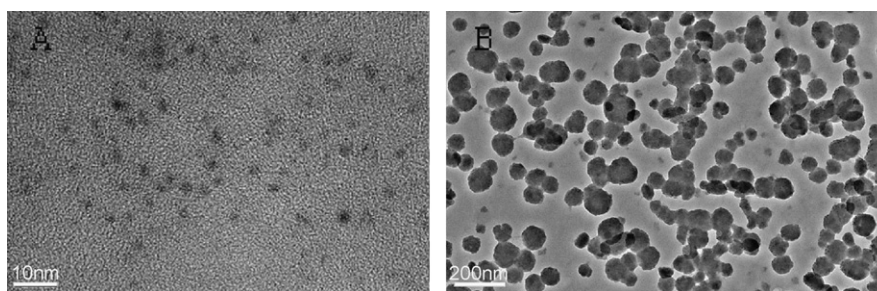
Fig. 3. The HRTEM images of the BSA-AuNCs (A), and the BSA-AuNCs in the presence of 5 \mu\text{M} nitrite (B).
