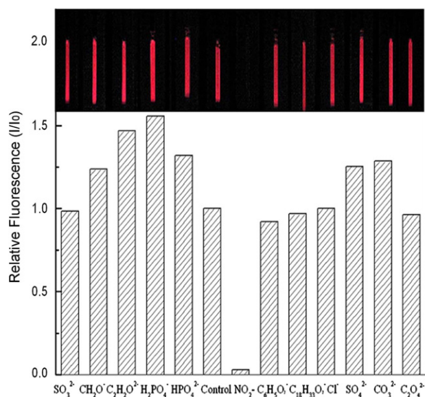
Fig. 2. Relative fluorescence ( I/I_0 ) of BSA-AuNCs solution in the presence of 50 \mu M various anions. Inset: Photographs of BSA-AuNCs solution in the presence of 50 \mu M various anion under UV light.
