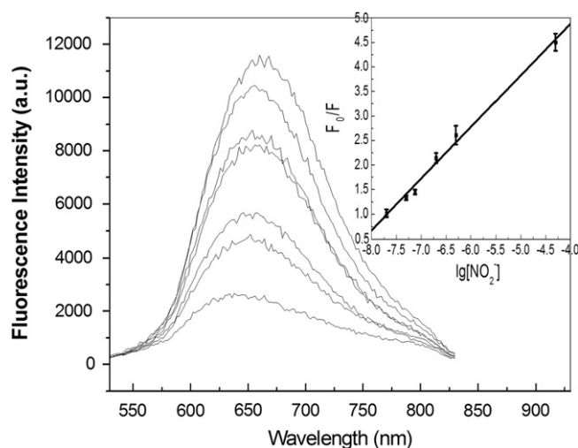
Fig. 5. Fluorescence emission spectra of BSA-AuNCs in the presence of different concentration of nitrite from 0 \mu\text{M} to 50 \mu\text{M} . Inset: Plot of the fluorescence intensity ratio of BSA-AuNCs at 670 nm versus the logarithmic of the concentration of nitrite.
